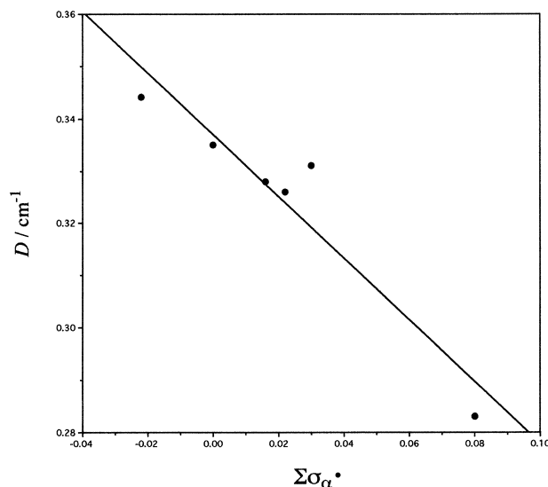
Fig. 2. The plot of the D values for bis(2,6-dimethyl-4- X -phenyl)carbenes 2 observed in TA at 200 K against \sigma_\alpha^\bullet .
