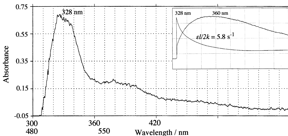
Fig. 4. Transient absorption spectra obtained in LFP of diazobis(2,6-dimethyl-4- tert -butylphenyl)methane ( 1c ) in degassed benzene with a 308-nm excimer laser recorded 1 \mu\text{s} after the pulse. Inset shows oscillogram traces monitored at 328 and 360 nm.
