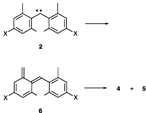
Scheme 4. Mechanism for the formation of 1,2-dihydrobenzocyclobutenes 4 and dihydroanthracenes 5 from triplet carbenes 2 .
