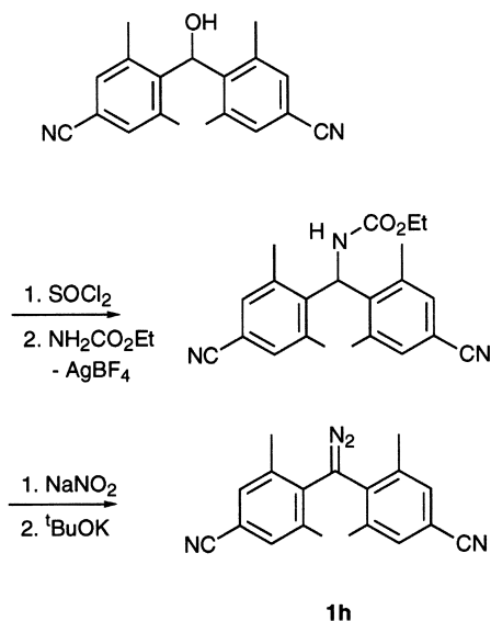
Scheme 2. Preparation of bis(2,6-dimethyl-4-cyanophenyl)diazomethane ( 1h ).
