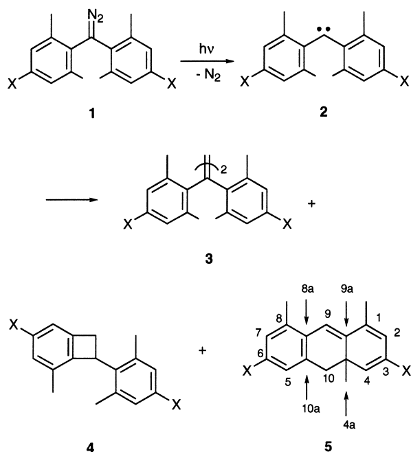
Scheme 3. Products obtained by photolysis of diazobis(2,6-dimethyl-4-X-phenyl)methanes ( 1a-h ) in degassed benzene.
