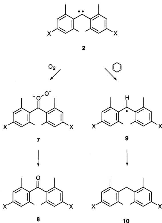
Scheme 5. Reactions of triplet carbenes 2 with oxygen and 1,4-cyclohexadiene.
