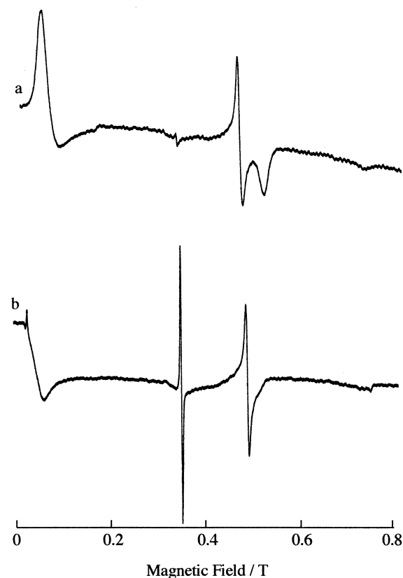
Fig. 1. ESR spectra of bis(4- t -butyl-2,6-dimethylphenyl)carbene ( 2c ) in 1,2,3-propanetriyl triacetate (PT). (a) Sample at 110 K. (b) Same sample after annealing to 190 K.
