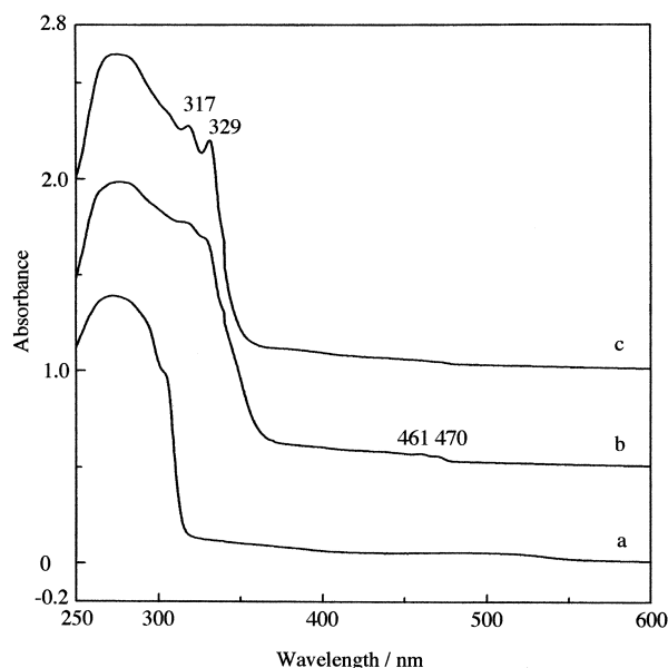
Fig. 3. UV/vis spectral changes observed in the photolysis of diazobis(2,6-dimethyl-4- tert -butylphenyl)methane ( 1c ). (a) UV/vis spectrum of 1c in 2-MTHF at 77 K. (b) Same sample after 10-min irradiation ( \lambda > 300 nm). (c) Same sample after thawing the matrix to 110 K.
